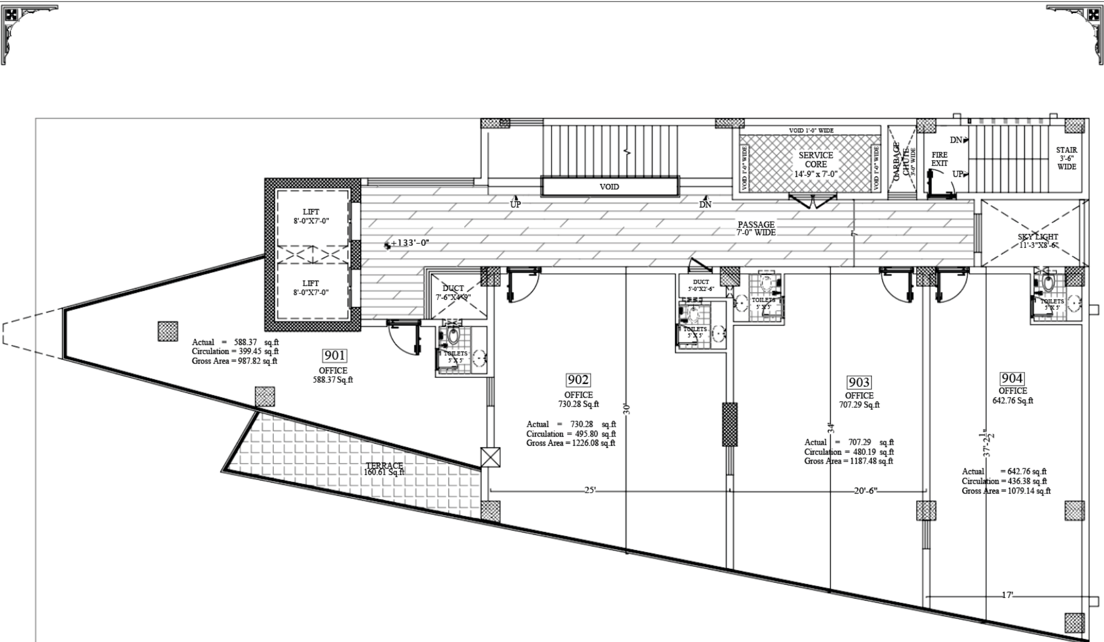
9th FLOOR PLAN ALL DIMENSIONS INCLUDING WALLS
