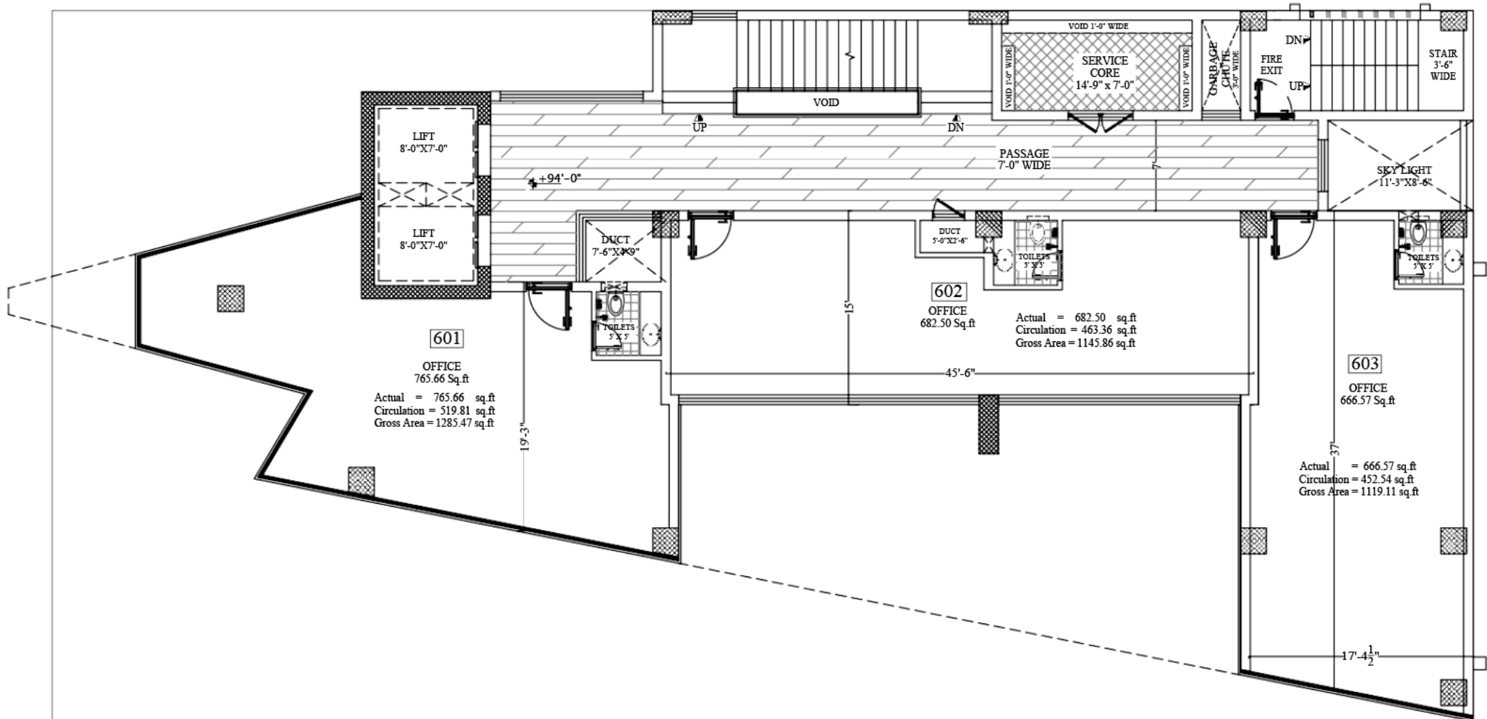
6th FLOOR PLAN ALL DIMENSIONS INCLUDING WALLS
