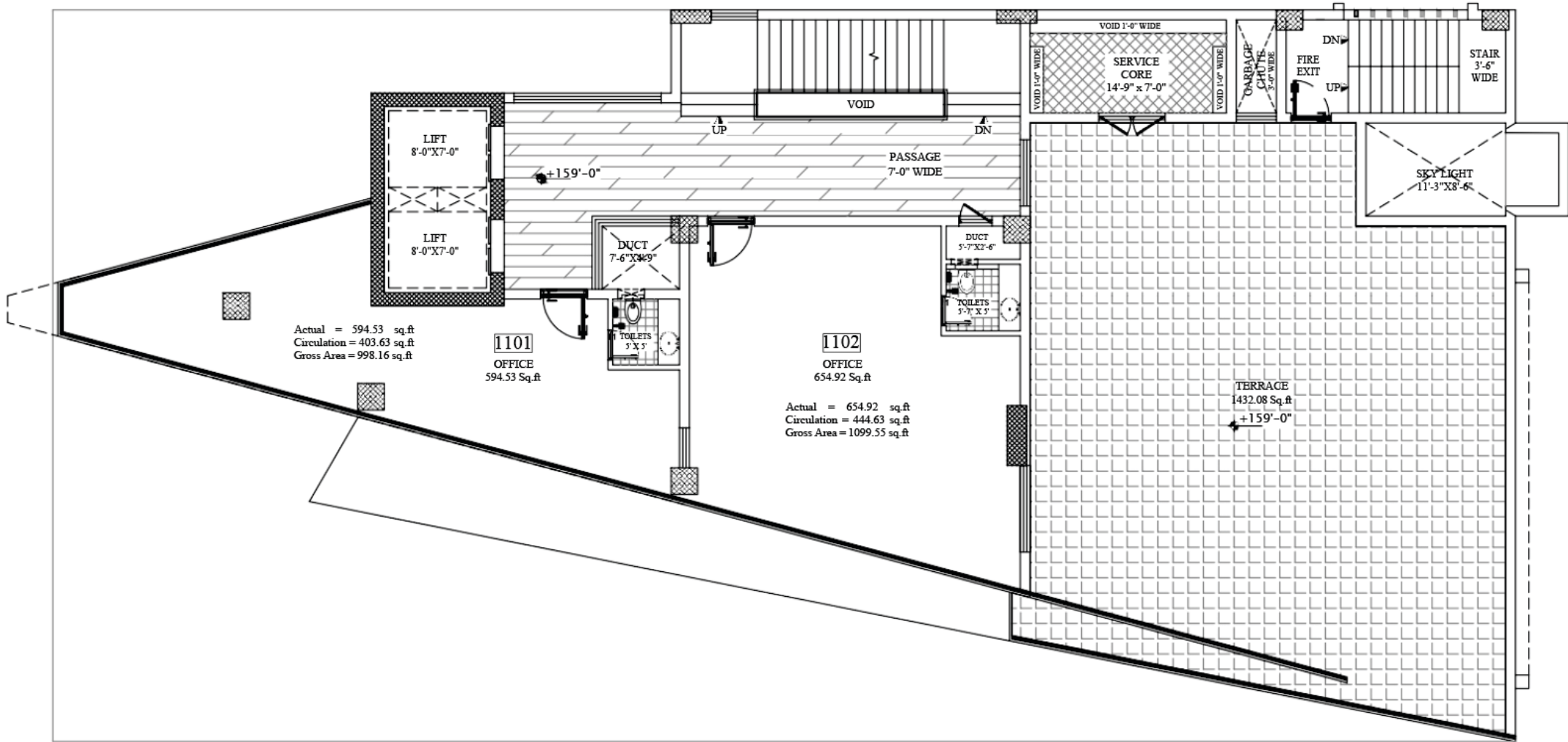
11th FLOOR PLAN ALL DIMENSIONS INCLUDING WALLS
