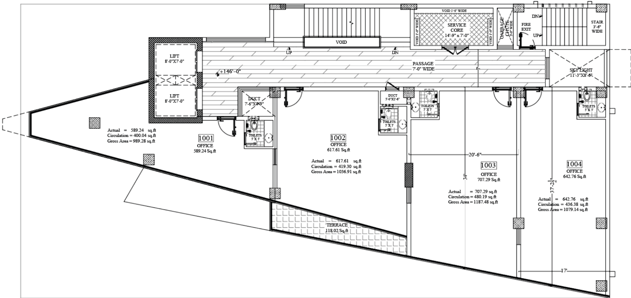
10th FLOOR PLAN ALL DIMENSIONS INCLUDING WALLS
