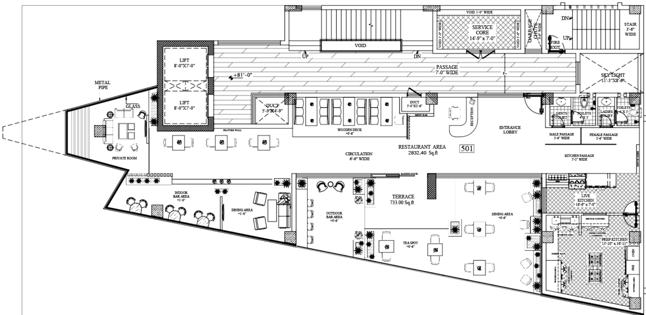
5th FLOOR PLAN ALL DIMENSIONS INCLUDING WALLS
