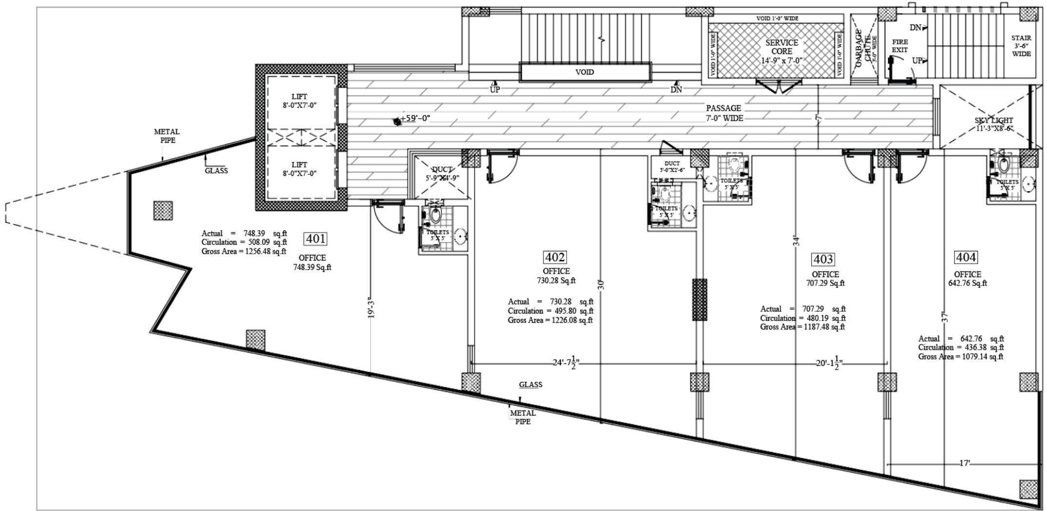
4th FLOOR PLAN ALL DIMENSIONS INCLUDING WALLS
