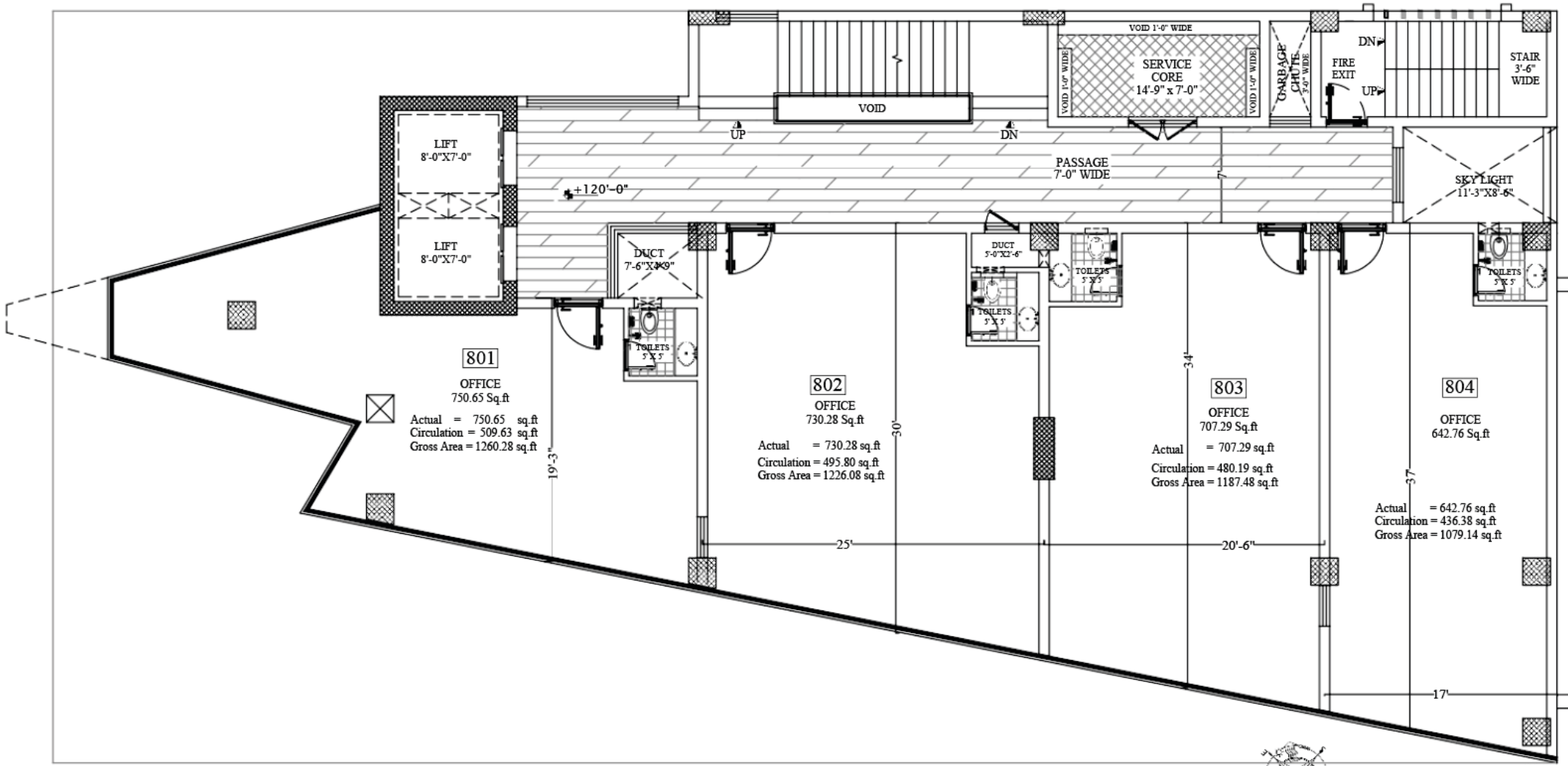
8th FLOOR PLAN ALL DIMENSIONS INCLUDING WALLS
