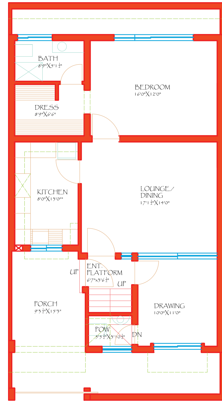
GROUND FLOOR PLAN COVERED AREA 1176 SQFT
